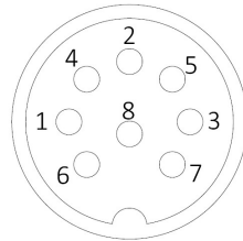
8Pin-A female
